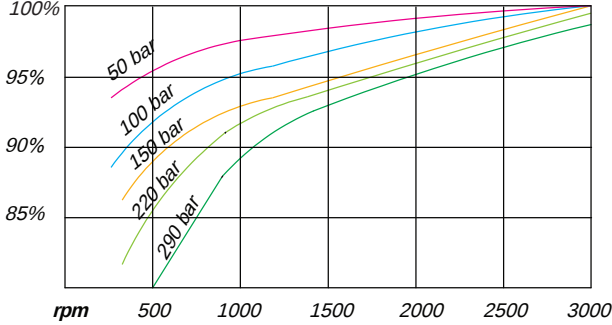
Hacimsel Verimlilik - Volumetric Efficiency
