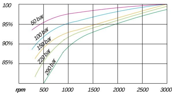
Hacimsel Verimlilik - Volumetric Efficiency
